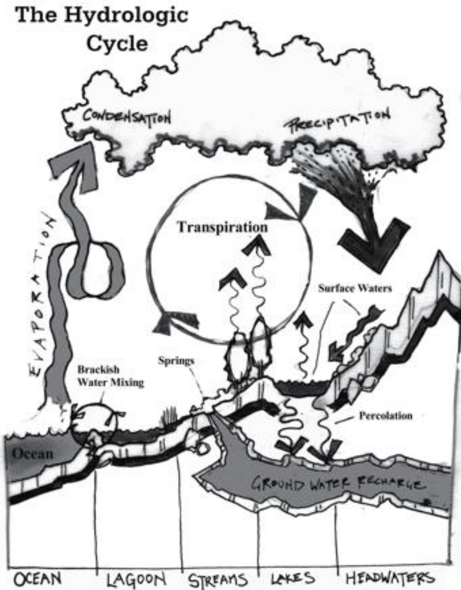
Figure 2-3. The Hydrologic Cycle.
